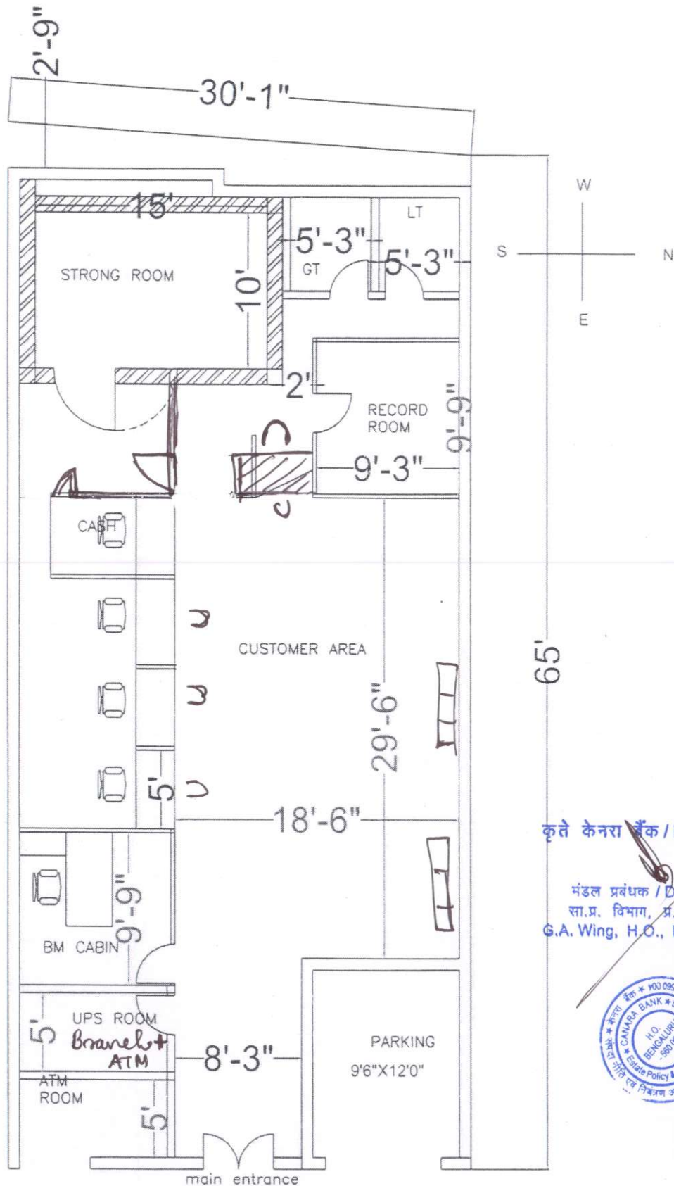
Proposed interior layout of Nawadih Dhanbad branch
